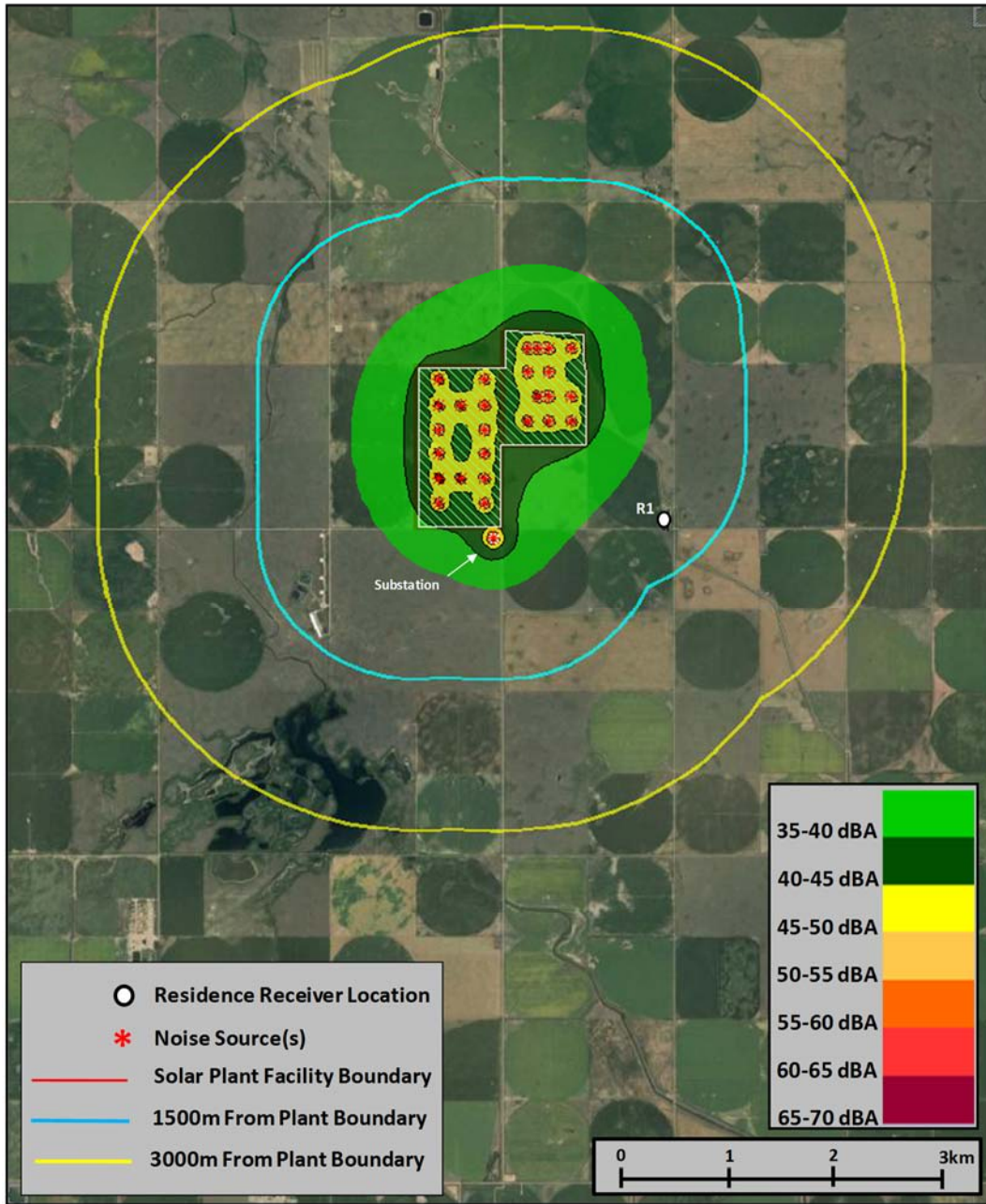
Figure 3 Facility Contribution Noise Contour Solar Krafte Prairie Sunlight I Solar Plant
